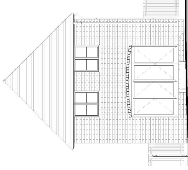
House 3/4 - West Elevation as Proposed 1 : 100
