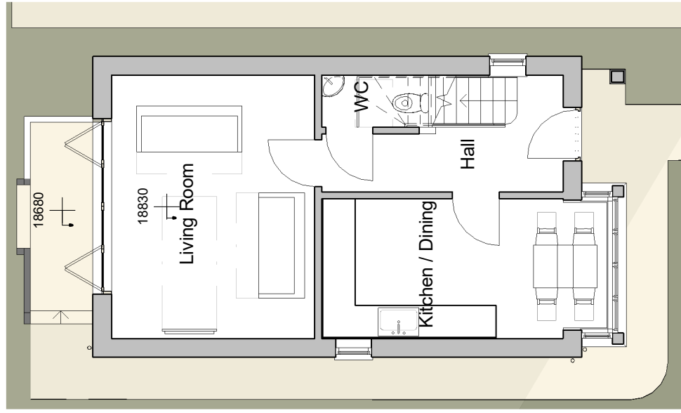
Houses 3/4 - Ground Floor Plan as Proposed 1 : 100
